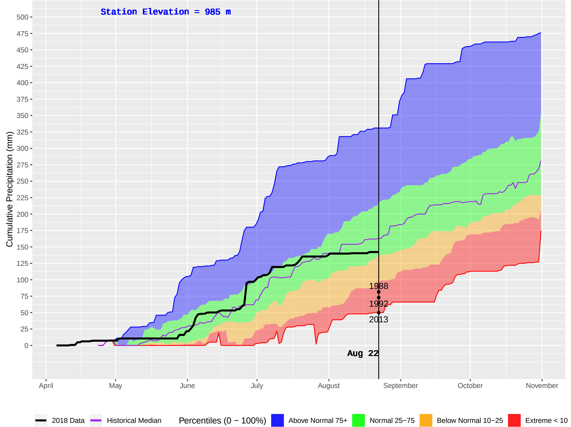
SIFTON (152) : Historical (1988–2016) and Current (2018) Daily Cumulative Precipitation
