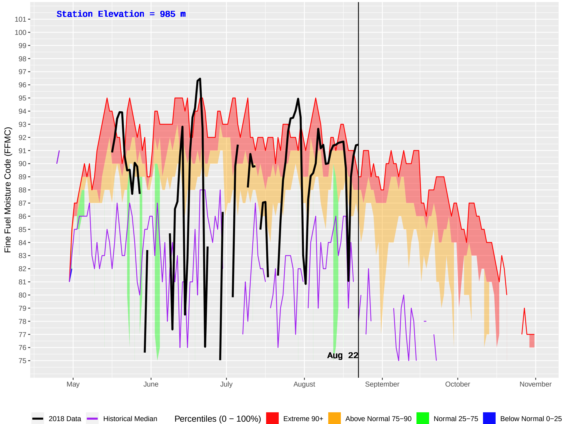
SIFTON (152) : Historical (1988–2016) and Current (2018) Daily Fine Fuel Moisture Code (FFMC)
